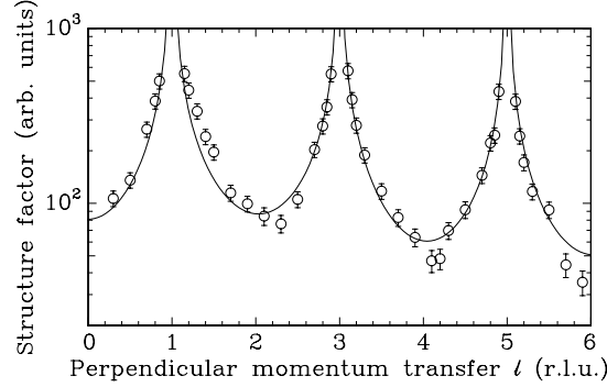
Figure 5.3: Structure factor amplitudes along the (1 2) crystal truncation rod of KDP(100). The solid curve is a calculation for a bulk terminated crystal with a rms roughness of 1.2 Å.
