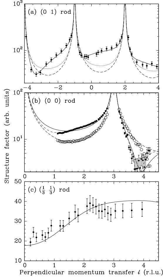
Figure 2.6: Structure-factor amplitudes along the (01), (00), and (\frac{1}{3} \frac{1}{3}) crystal truncation rods for Cu(111)( \sqrt{3} \times \sqrt{3} )R30°-Sb. Measured structure factors are indicated by filled circles. The open circles in (b) are measurements of clean Cu(111). The dashed curves give the calculation for the bulk-terminated Cu(111) surface and the solid curves represent best-fit model calculations. In (a) the dotted curve represents a calculation for a structural model where the Sb atom is at a “normal” substitutional fcc site. For the specular rod in (b) the dashed-dotted curve represents a calculation with an extra Sb atom on top of the surface (see text).
